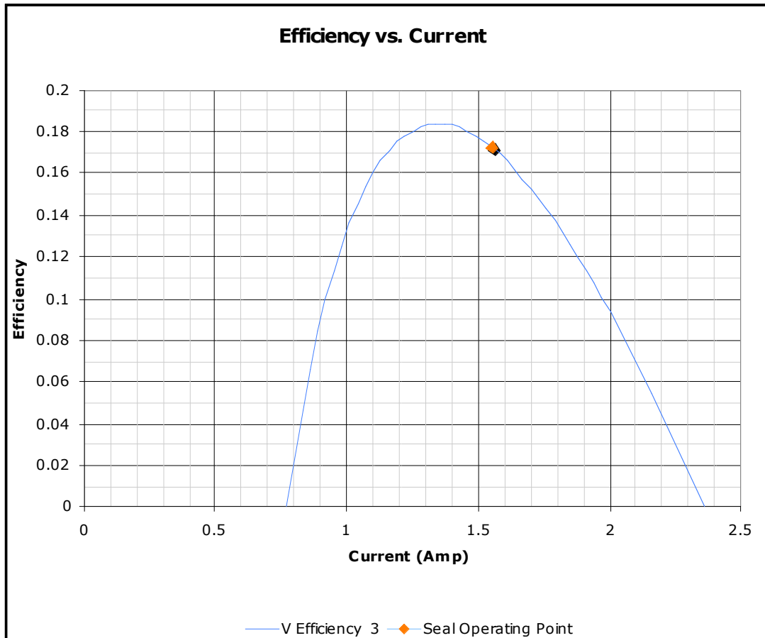
Figure 1: Efficiency vs. Current plot with seal's operating point
